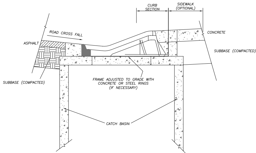
SECTION VIEW PARALLEL TO CURB
