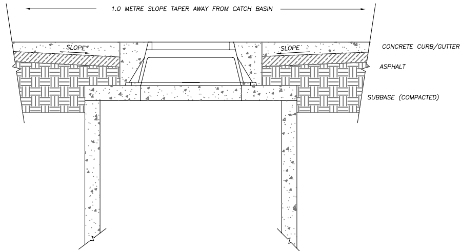
SECTION VIEW PERPENDICULAR TO CURB
